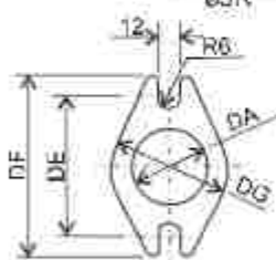
Oval flange
