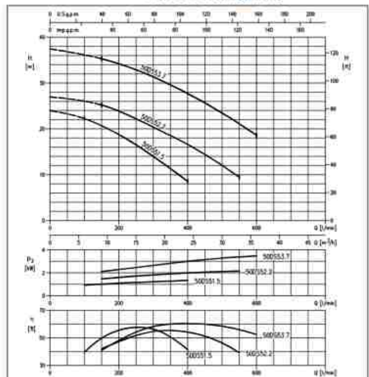
PERFORMANCE CURVES series 50DS51.5 (1.5 kW) series 50DS52.2 (2.2 kW) series 50DS53.7 (3.7 kW)
