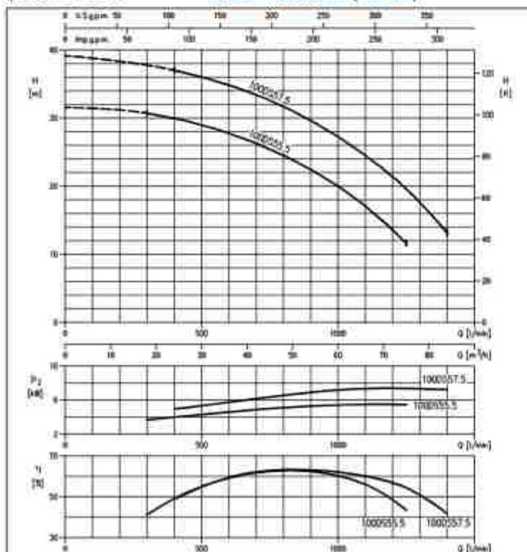
PERFORMANCE CURVES series 100DS55.5 (5.5 kW) series 100DS57.5 (7.5 kW) (per ISO 9906 Annex A)
