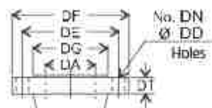
Round flange
