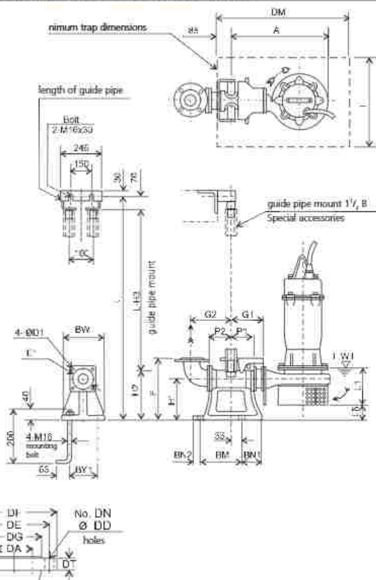
DIMENSIONS DS with ODC (lowering device) (5.5 - 7.5 kW)
