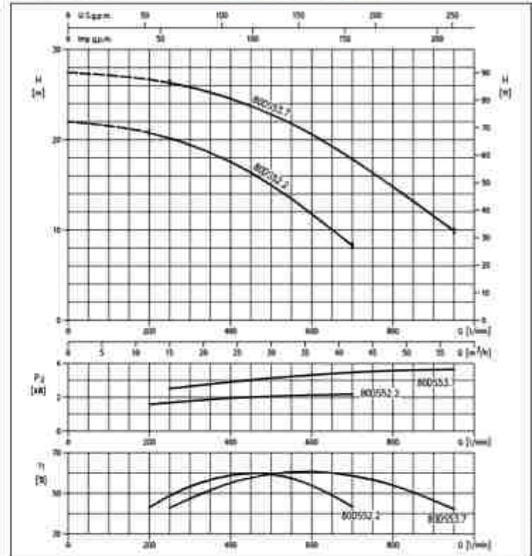
PERFORMANCE CURVES series 80DS52.2 (2.2 kW) series 80DS53.7 (3.7 kW) (per ISO 9906 Annex A)
