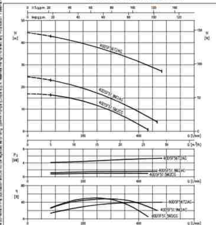
PERFORMANCE CURVES series 40DSF51.5M2CG (1.5 kW) series 40DSF51.9M2AG (1.9 kW) series 40DSF56T2AG (6.0 kW)
